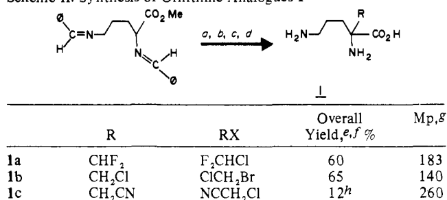
Scheme II. Synthesis of Ornithine Analogues 1
